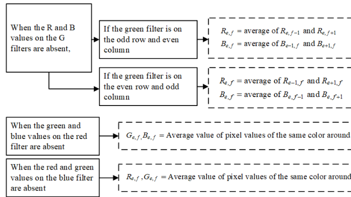
Figure 2. Mechanism of bilinear interpolation algorithm.
